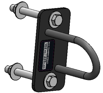
XR16-02 ROPE ANCHOR
